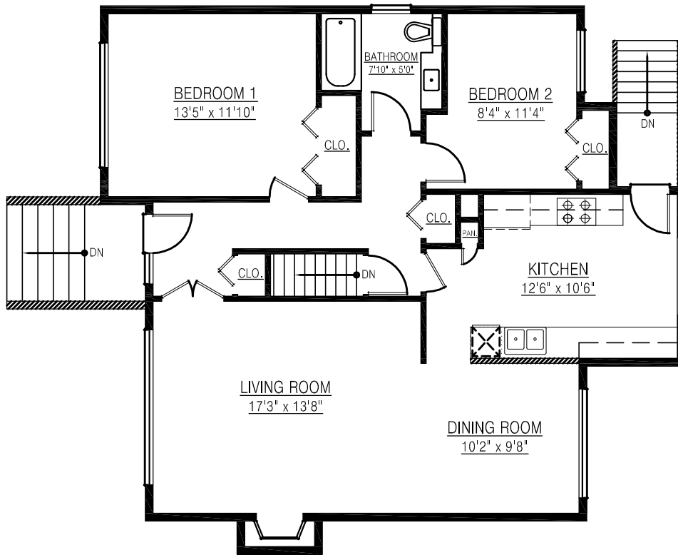
MAIN FLOOR PLAN FLOOR AREA: 1075 sq.ft.
