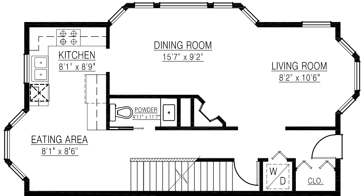
MAIN FLOOR PLAN FLOOR AREA: 656 sq.ft.
