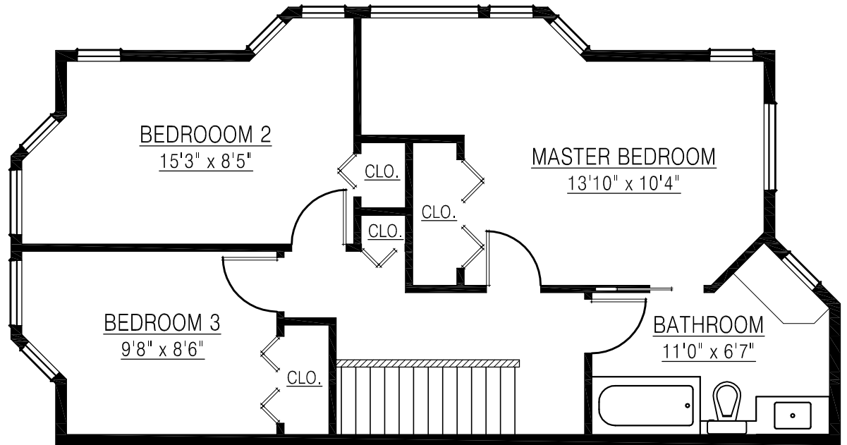
UPPER FLOOR PLAN FLOOR AREA: 678 sq.ft.
