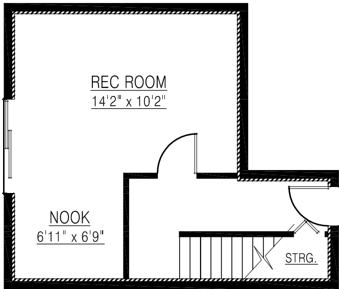
LOWER FLOOR PLAN FLOOR AREA: 327 sq.ft.
